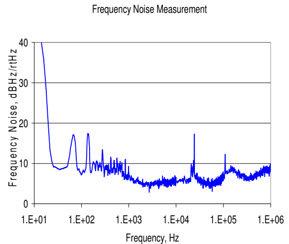
Frequency noise measurement plot
